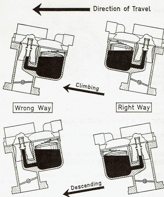
Fig. 4 Position of the Float Chamber
