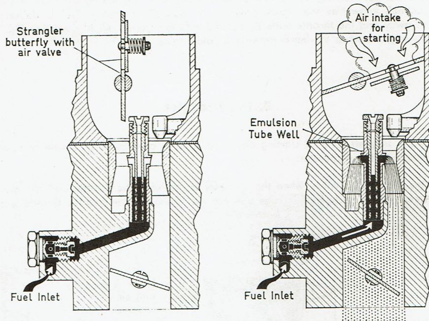
Fig. 14 Strangler Butterfly with Air Valve
