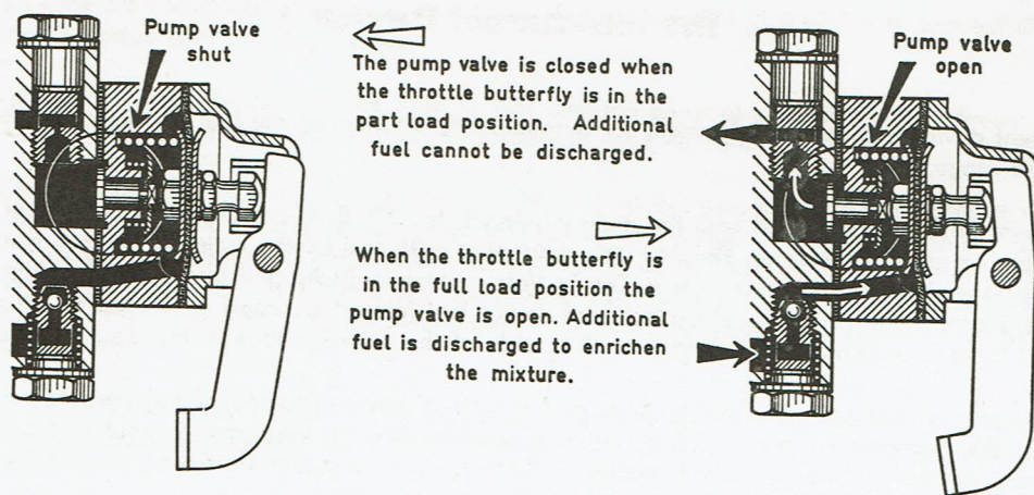
Fig. 35 "Rich" pump with disc valve (pump 83)
