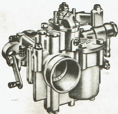
Type 32 HR (Horizontal Carburetor)
