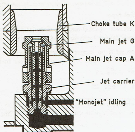
Fig. 23 Assembly No. 12
