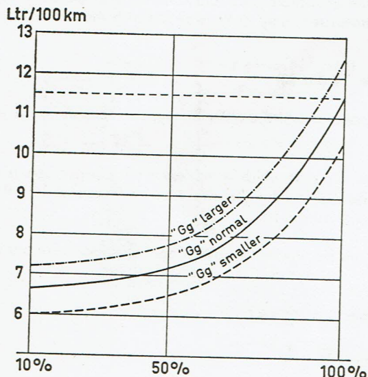
Fig. 21 Diagram of the affect of the main jet Gg
