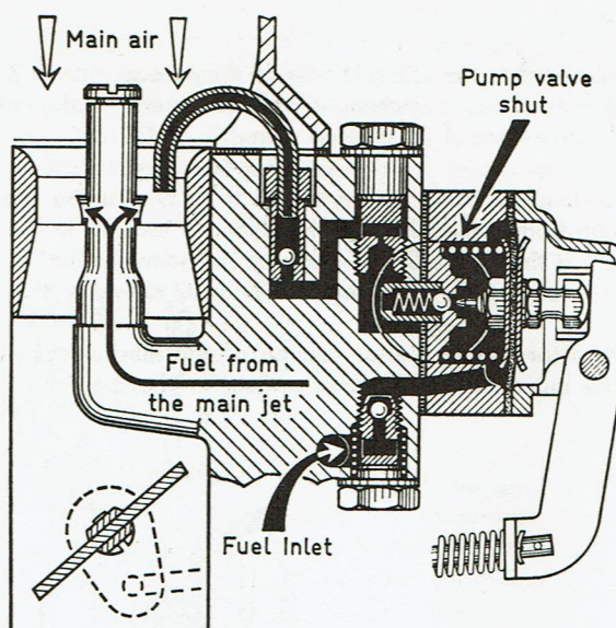
Fig. 34 "Rich" pump with ball valve (pump 73)
