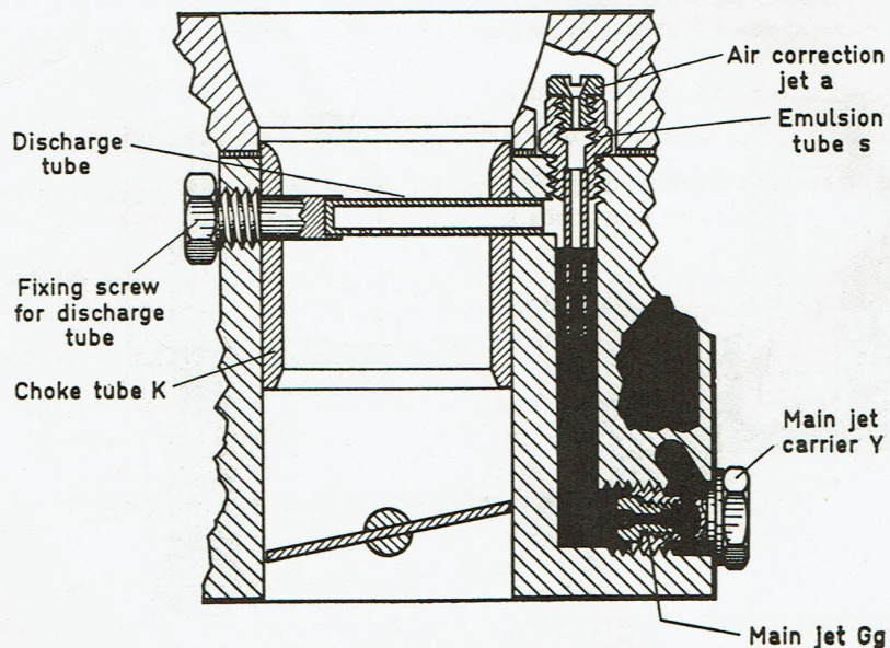
Fig. 28 Jet assembly of the 40 PII carburetor
