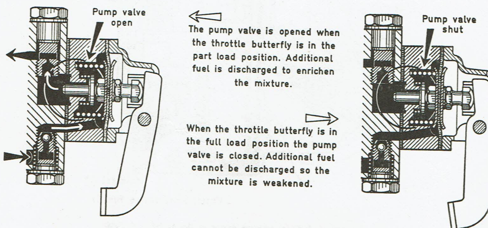
Fig. 36 "Weak" pump with disc valve (pump 84)
