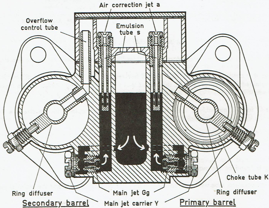
Fig. 27 Jet assembly of the 44 PHH carburetor
