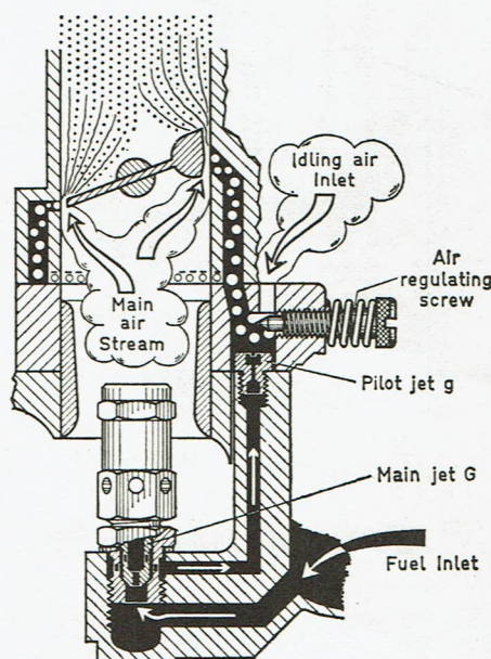
Fig. 17 Idling with air control
