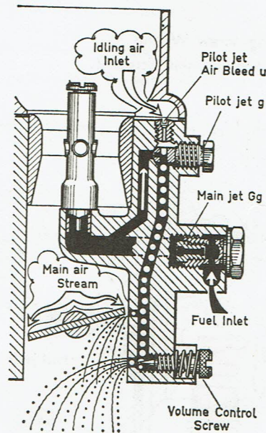
Fig. 16 Idling with mixture control
