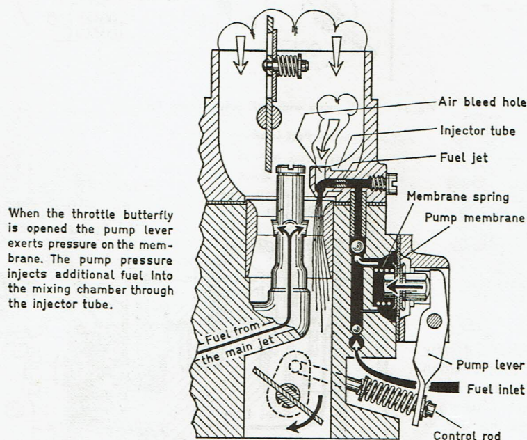
Fig. 33 Accelerator pump of the 28 PCI carburetor
