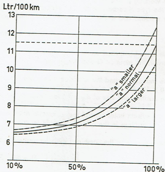
Fig. 22 Diagram of the affect of the air correction jet a
