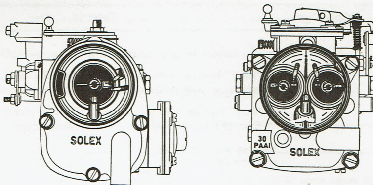
Fig. 3 Types of carburetors
