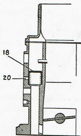
Fig 2 Starter in action (after starting)
