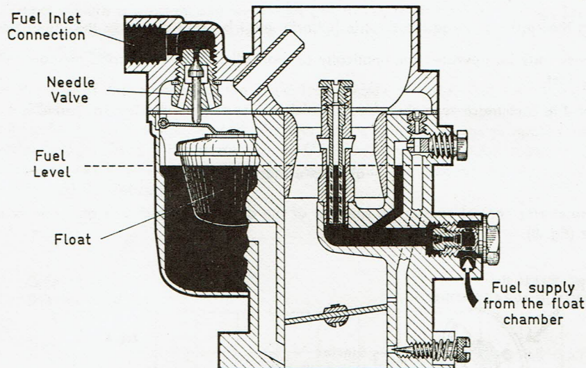
Fig. 6 The Float System
