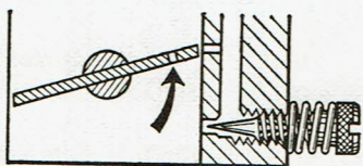
c) A hole in the throttle butterfly causes the "by-pass" orifice to discharge slower.
