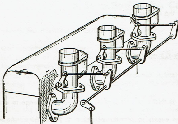
Fig. 5 Control layout for multiple carburetors
