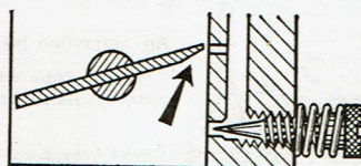
d) A bevelled edge on the throttle butterfly causes the "by-pass" orifice to discharge earlier.
