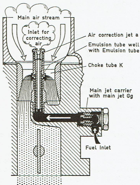
Fig. 19 Main jet circuit of a downdraught carburetor
