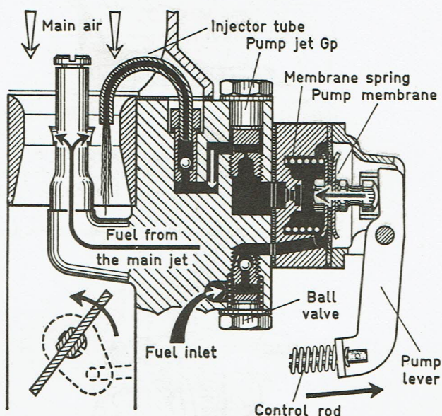
Fig. 29 Mechanically operated accelerator pump
