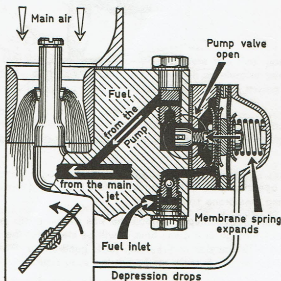
Fig. 30 Depression operated accelerator pump
