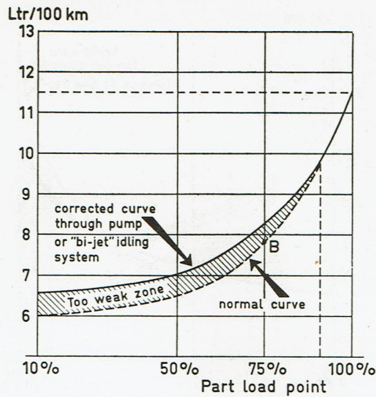
Fig. 40 Influence of the "weak" pump or of a "bi-jet" idling system
