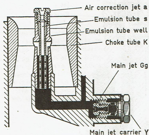
Fig. 25 Assembly No. 21
