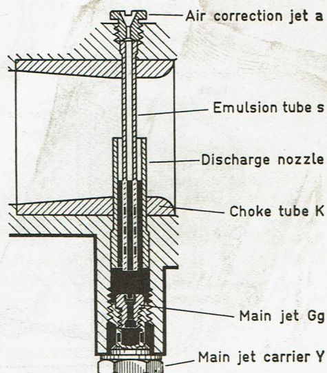
Fig. 26 Assembly No. 22
