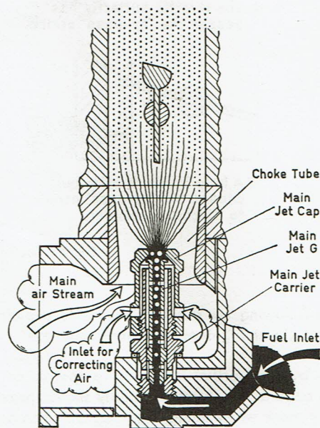
Fig. 20 Main jet circuit of a updraught carburetor
